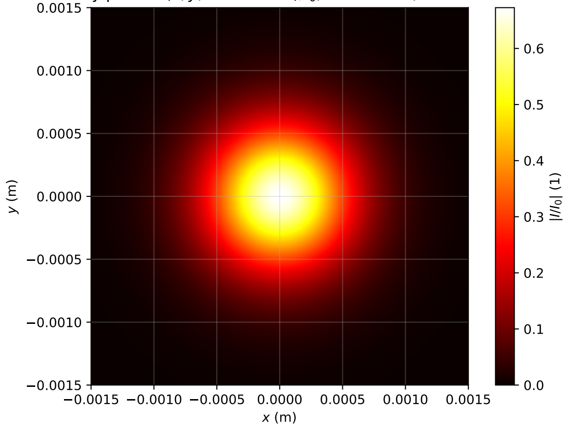
Intensity profile I(x, y, z = 2.548m)/I_0 , P_{in}=0.5P_{cr} , artificial time
